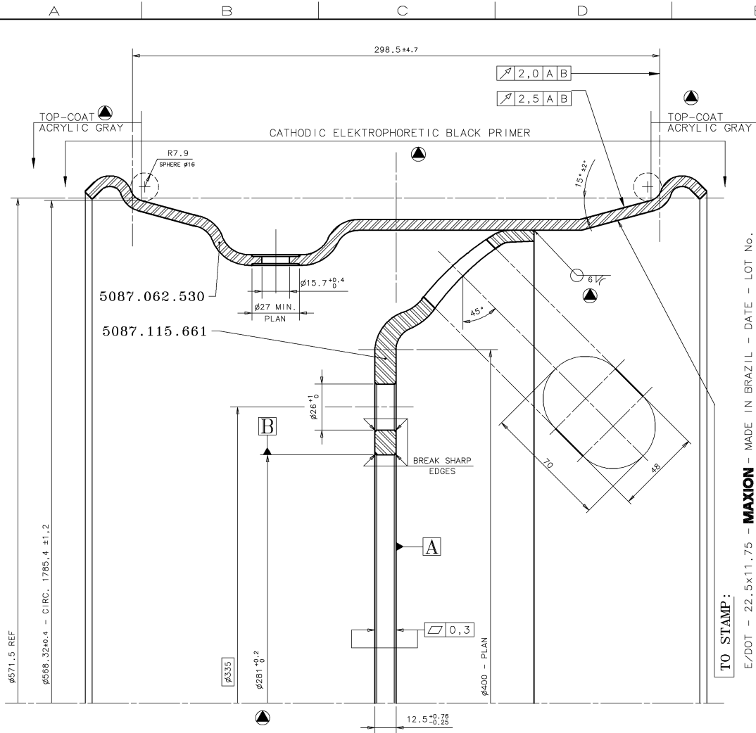
SECTION - CC
